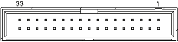
Figure 4. MXP Pinout
